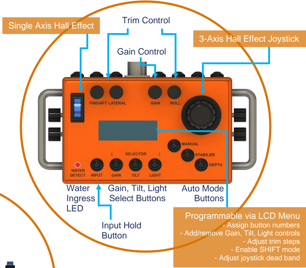
IP67 USB Hand Control Unit
